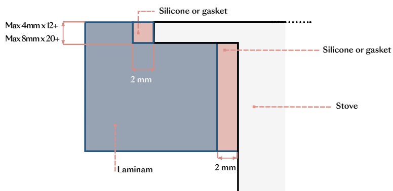
Stove flush with the countertop
